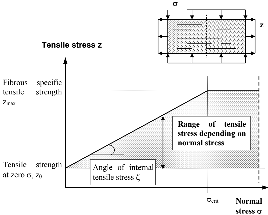
Fig. 4: Failure characteristics of fibrous waste material in tension test under normal load
