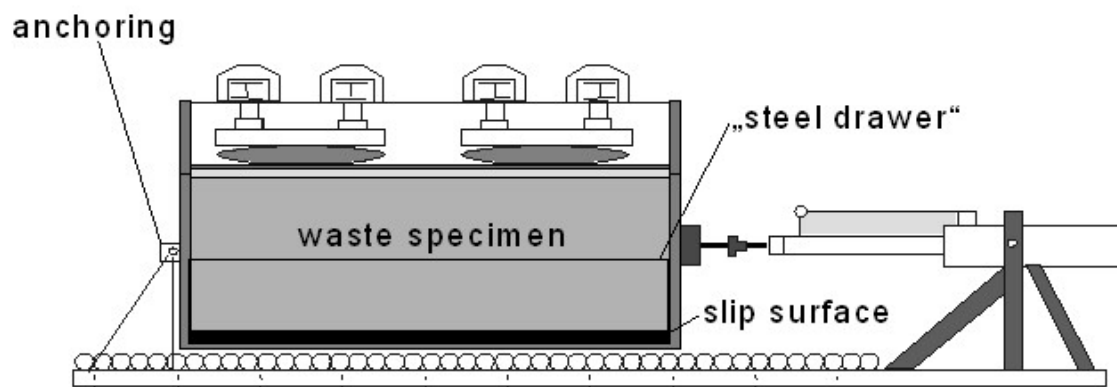
Fig. 7: Large shear test – equipment
