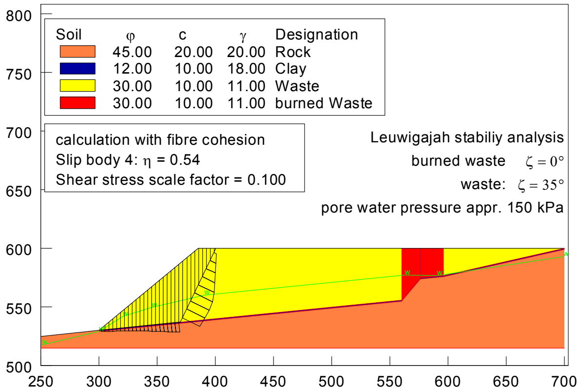
Fig. 18: Stability analysis according to the common method
