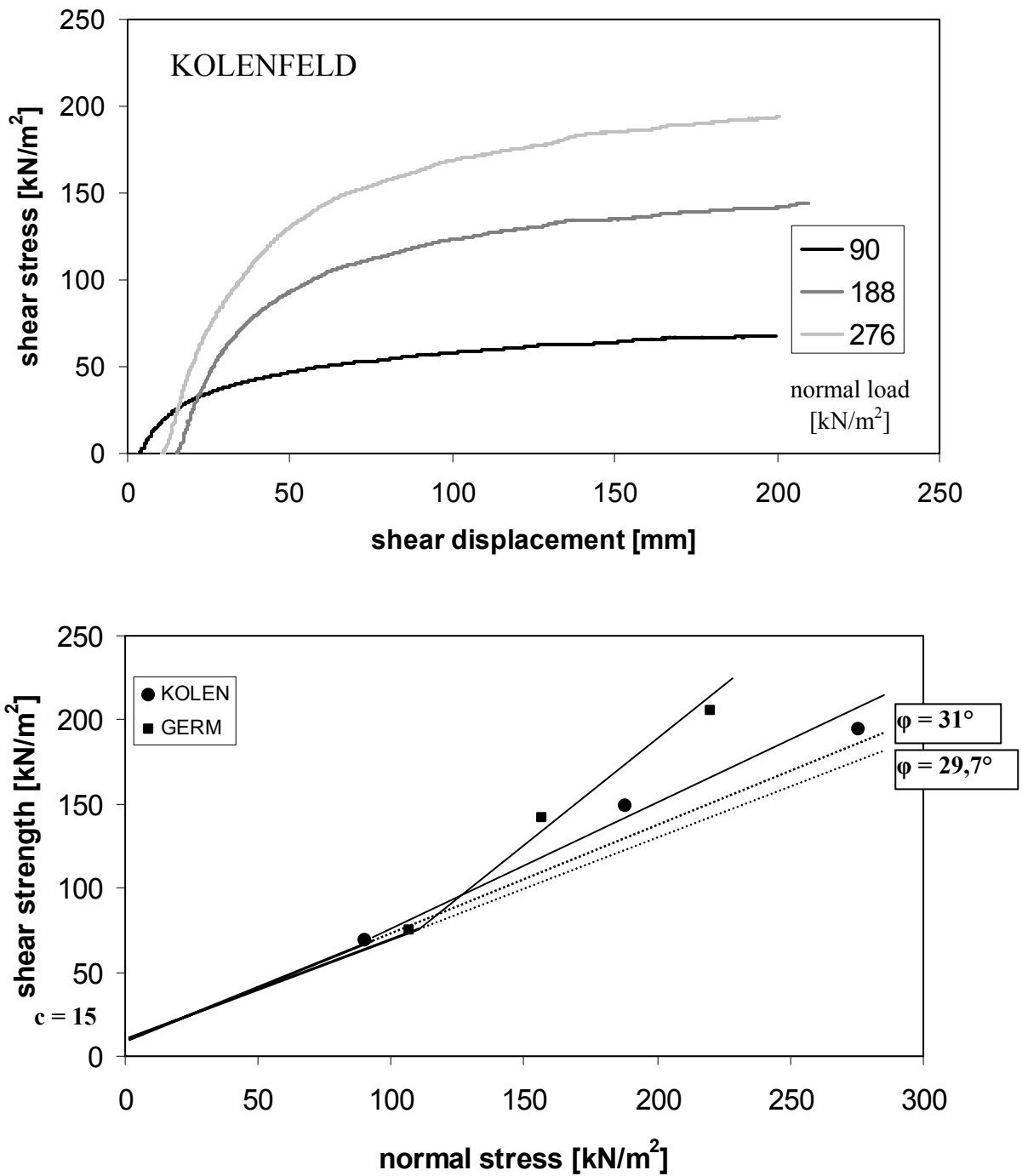
Fig 9: Direct shear test on MSW – results: stress-strain (left), non linear shear planes (right)
