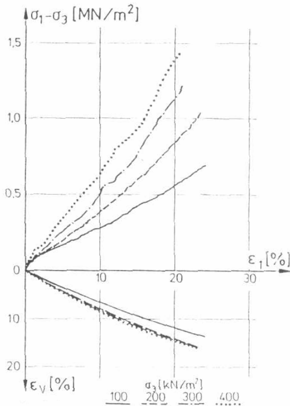
Fig. 10: results of triaxial compression test by Jessberger et al. (1995)
