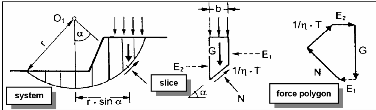
Fig. 16: Bishop method of slices
