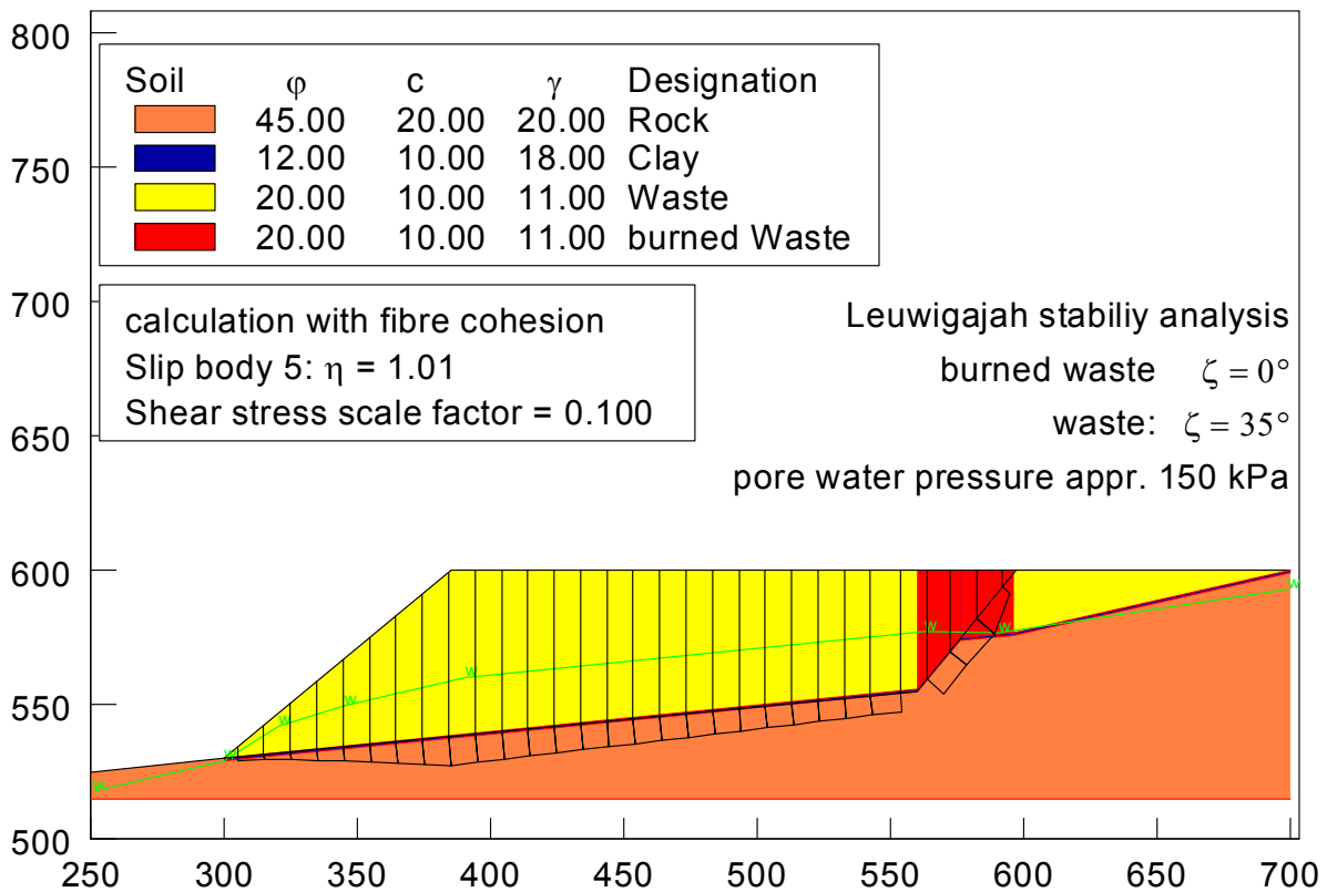
Fig. 17: Stability analysis according to the advanced method of fiber-cohesion
