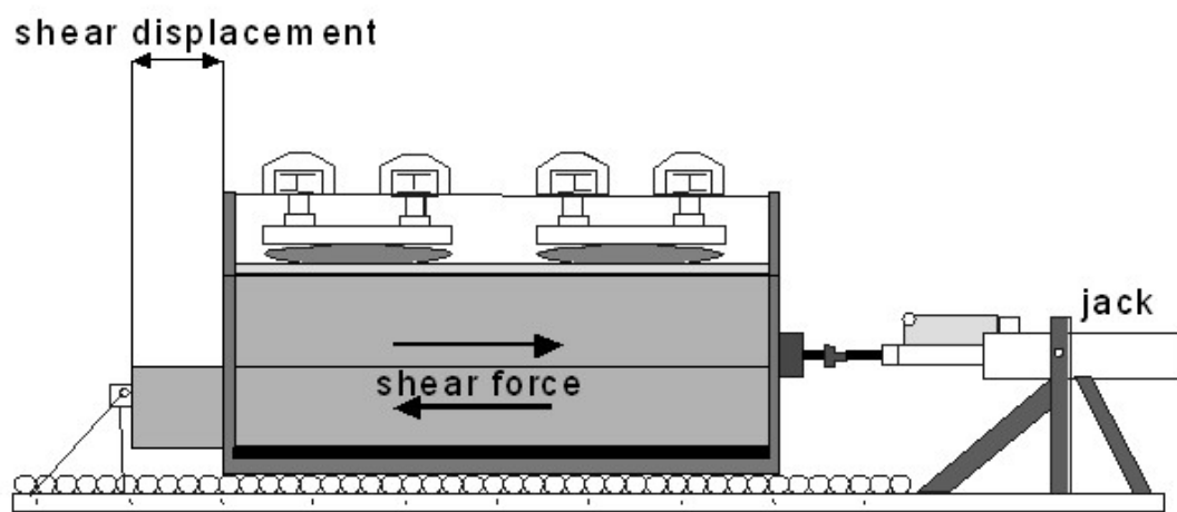
Fig. 8: Large shear test – testing procedure
