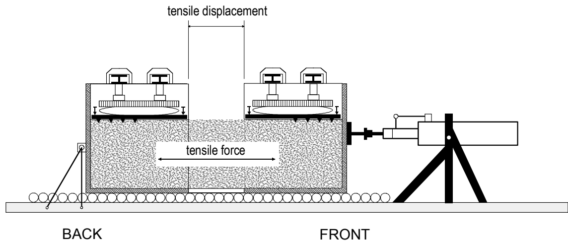
Fig. 5: Tension test under normal load – principle and procedure
